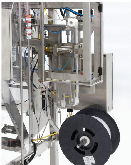
Optional transverse zipper applicator is integrated into the film cage
