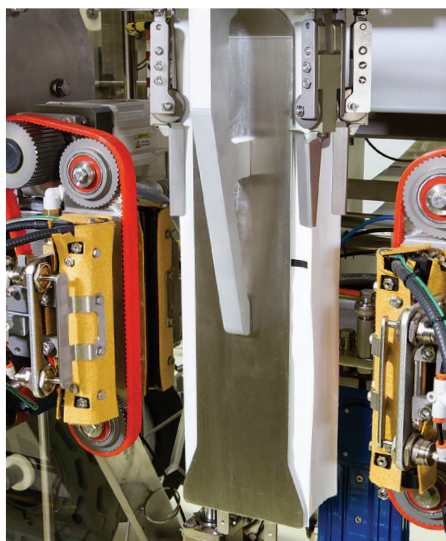
Optional square forming tube produces quad-seal bags with crisp corner seals
